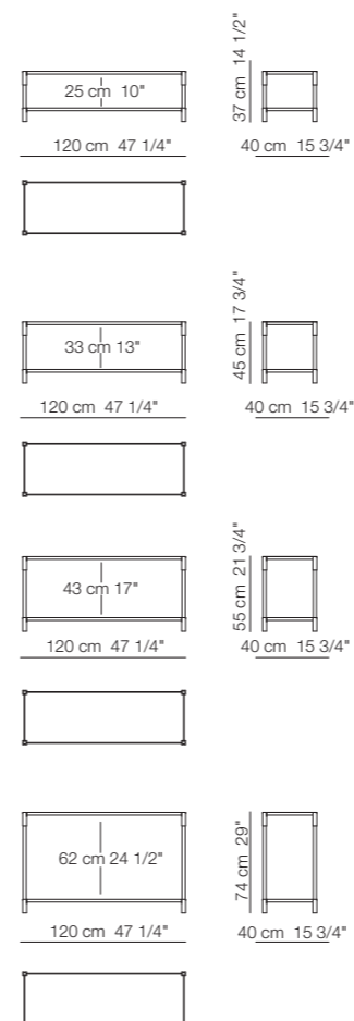
Moduli per base librerie Elements for bookcase base
