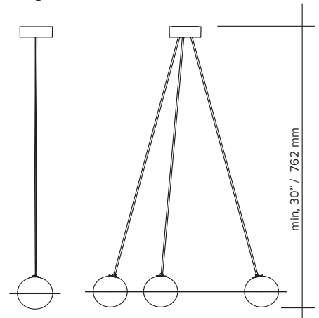
angled wires
