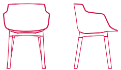
4-legged CROSS and OAK CROSS base L55 D54 H76.4 cm seat H44 cm armrest H67 cm
